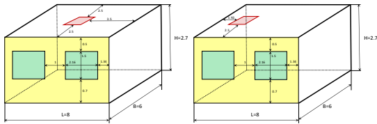
Figure 5. Scheme of small radiant heater centered (left) and acentric (right).
