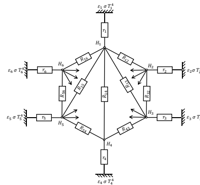
Figure 3. Model for long-wave radiation exchange with 6 surfaces
