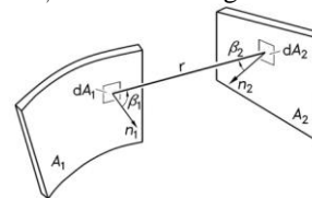
Figure 4. Calculation of View Factor [15]
