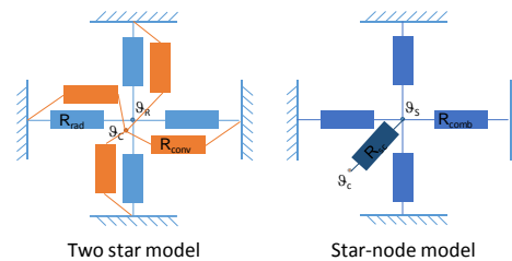
Figure 1. star-node model (right) and two-star model (left) with four surfaces: \vartheta_r radiative node, \vartheta_c convective node, \vartheta_s star node (mixture of surface and air temperature), R_{rad} radiative resistance, R_{conv} convective resistance, R_{comb} combined radiative and convective resistance and R_{sc} the resistance between the star node and the convective node
