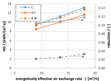
Figure 7. Heating demand (HD) for the small radiant heater on the ceiling (R C) and wall (R W) and reduction with respect to convective heating (C) depending on the energetically effective air exchange rate
