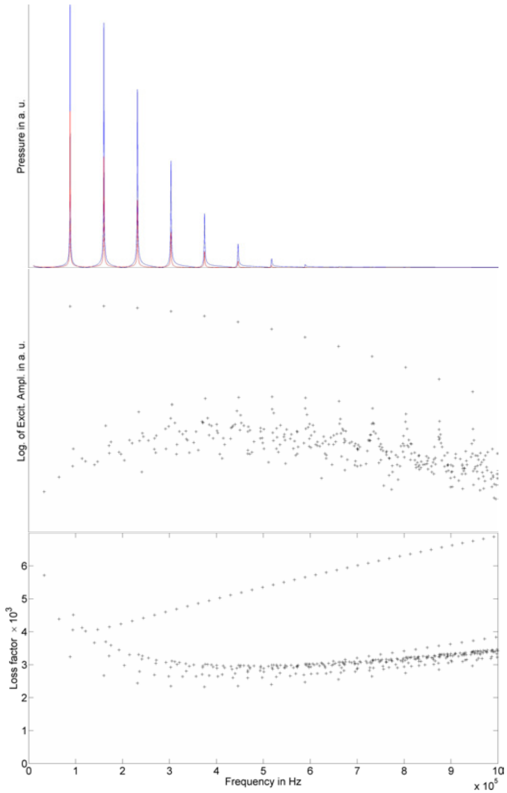
Fig. 2: Response function in arbitrary units at two different locations inside the arc tube (top), logarithm of excitation amplitudes according to Equation (12) in arbitrary units (middle) and total loss factor times 10^3 (bottom) as function of the frequency in Hz.
