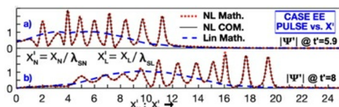
Figure 1 : Figure 1 EEPulse Into Field at rest : |\Psi'| & \text{re } \Psi' vs. x_N' ; x_L'
