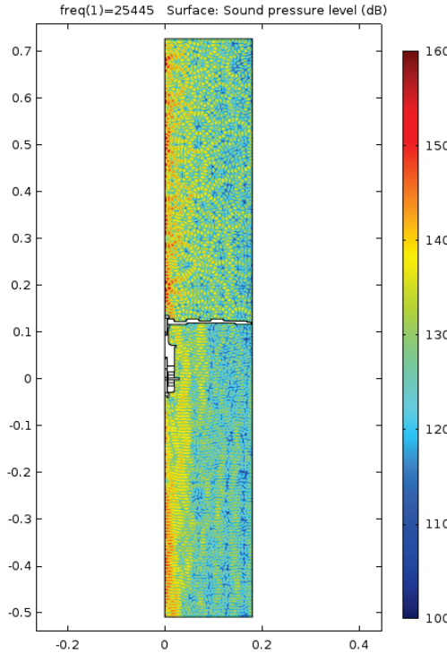
Figure 10. Acoustic pressure level (dB) in the dehydration chamber.
